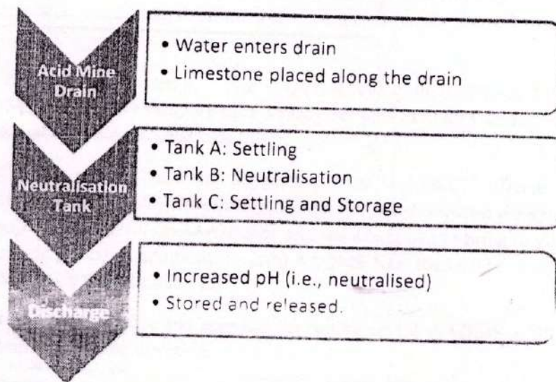
Fig 2: Flowchart depicting the AMD and the constructed Neutralisation Tank.
